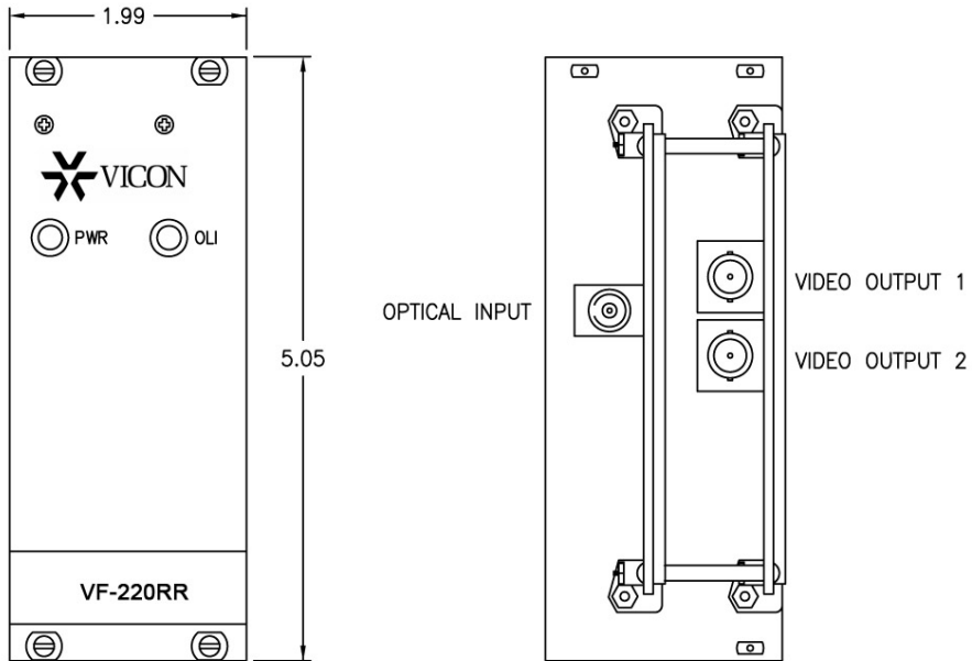
VF-220RR Rack-Mount Receiver
