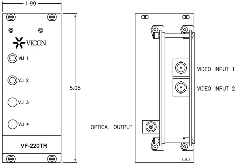
VF-220TR Rack-Mount Transmitter
